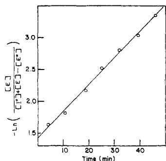
FIGURE 2: Determination of k_3 at pH 4.62; in 4.05 mM L-cysteine, 0.405 mM EDTA, \Gamma/2 = 0.12 , 10% ethanol, 25°. [E^0] = 10 \mu\text{M} , [I^0] = 45 \mu\text{M} .
