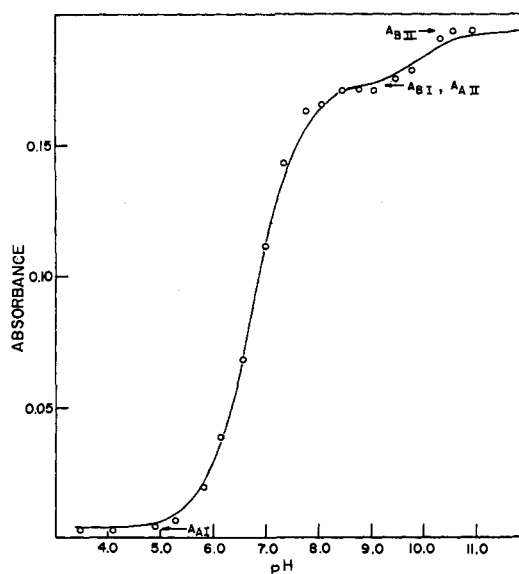
FIGURE 8: Spectrophotometric titration curve for 12.9 \mu\text{M} papain-R at 410 nm. Conditions were the same as in Figure 7. Solid line is a calculated titration curve for two acidic groups pK_I = 6.79 , pK_{II} = 10 . With A_{AI} = 0.003 , A_{BI} = A_{AII} = 0.173 , and A_{BII} = 0.194 .
