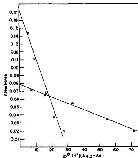
FIGURE 5: Determination of the ionization constant of the reporter group in 2 at 5.00 \mu\text{M} 2 : (●) and in papain-R at 12.9 \mu\text{M} papain-R; (○) using eq 10. A_A was set at 0.0018 and 0.0030 for 2 and papain-R, respectively.
