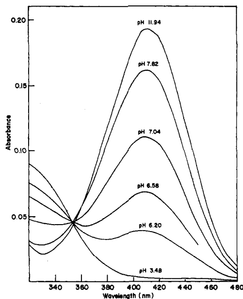
FIGURE 7: Dependence of the spectrum of papain-R on pH. At 12.9 \mu\text{M} papain-R, 25^\circ , \Gamma/2 = 0.145 .
