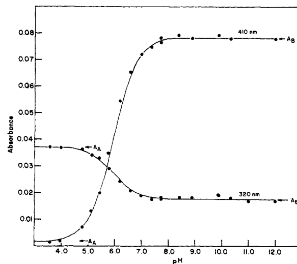
FIGURE 4: Spectrophotometric titration of 5.00 \mu\text{M} 2 at 320 and 410 nm. Conditions were the same as in Figure 3. Solid lines calculated from eq 10 with K = 10^{-5.92} , A_A = 0.0018 and A_B = 0.0784 at 410 nm, and A_A = 0.0370 and A_B = 0.0176 at 320 nm.
