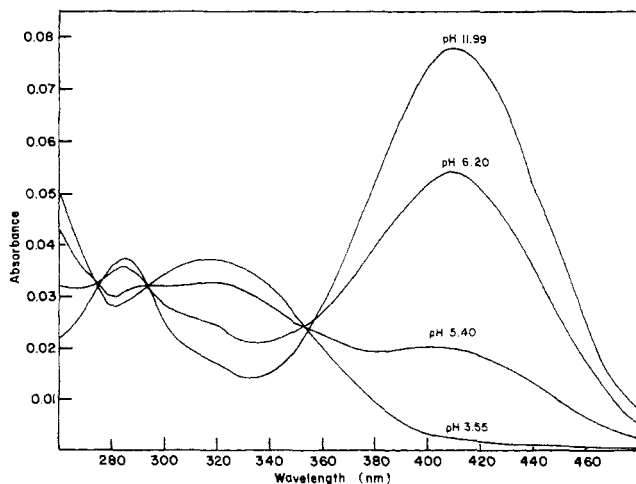
FIGURE 3: Dependence of the spectrum of model compound 2 on pH. At 5.00 \mu\text{M} 2 , 25°, \Gamma/2 = 0.145 .
