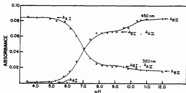
FIGURE 9: Spectrophotometric titration curves for 12.9 \mu M papain-R at 320 and 450 nm. Solid lines are calculated titration curves for two acidic groups, pK_I = 6.79 , pK_{II} = 10 , with A_{AI} = 0.084 , A_{BI} = A_{AII} = 0.022 , and A_{BII} = 0.016 at 320 nm, and A_{AI} = 0.001 , A_{BI} = A_{AII} = 0.066 , and A_{BII} = 0.083 at 450 nm.
