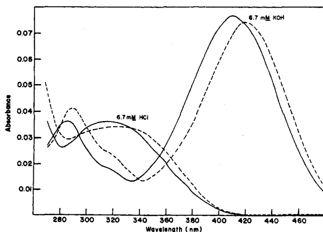
FIGURE 6: Effect of dioxane on the spectrum of the reporter group in 2 : (---) 33% dioxane; (—) water. \Gamma/2 = 0.0965 , 5.00 \mu\text{M} 2 .
