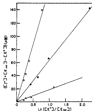
FIGURE 1: Determination of the ratio (k_1 + k_2^0)/k_3 , pH 5.63; ( \Delta ) pH 6.52, ( \bullet ) pH 7.20, ( \circ ) in 4.05 mM L-cysteine, 0.405 mM EDTA, \Gamma/2 = 0.12 , 10% ethanol, 25°, [E^0] = 9 –18 \mu\text{M} .
